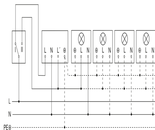
Circuit diagram Connection via a changeover switch for continuous and automatic operation
