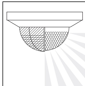
Vertical separation = reduction of the angle of coverage
